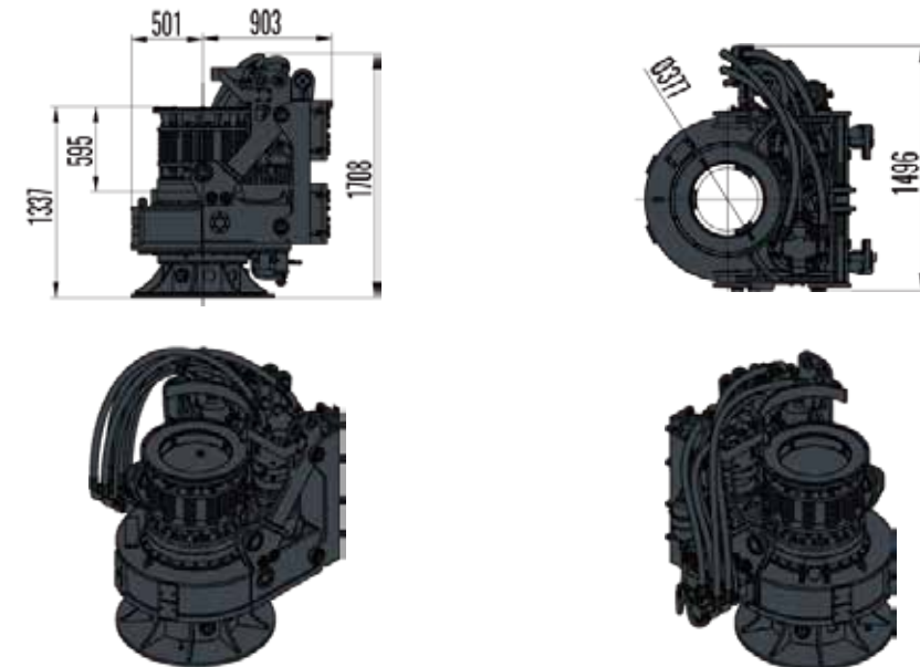
Rotary head
