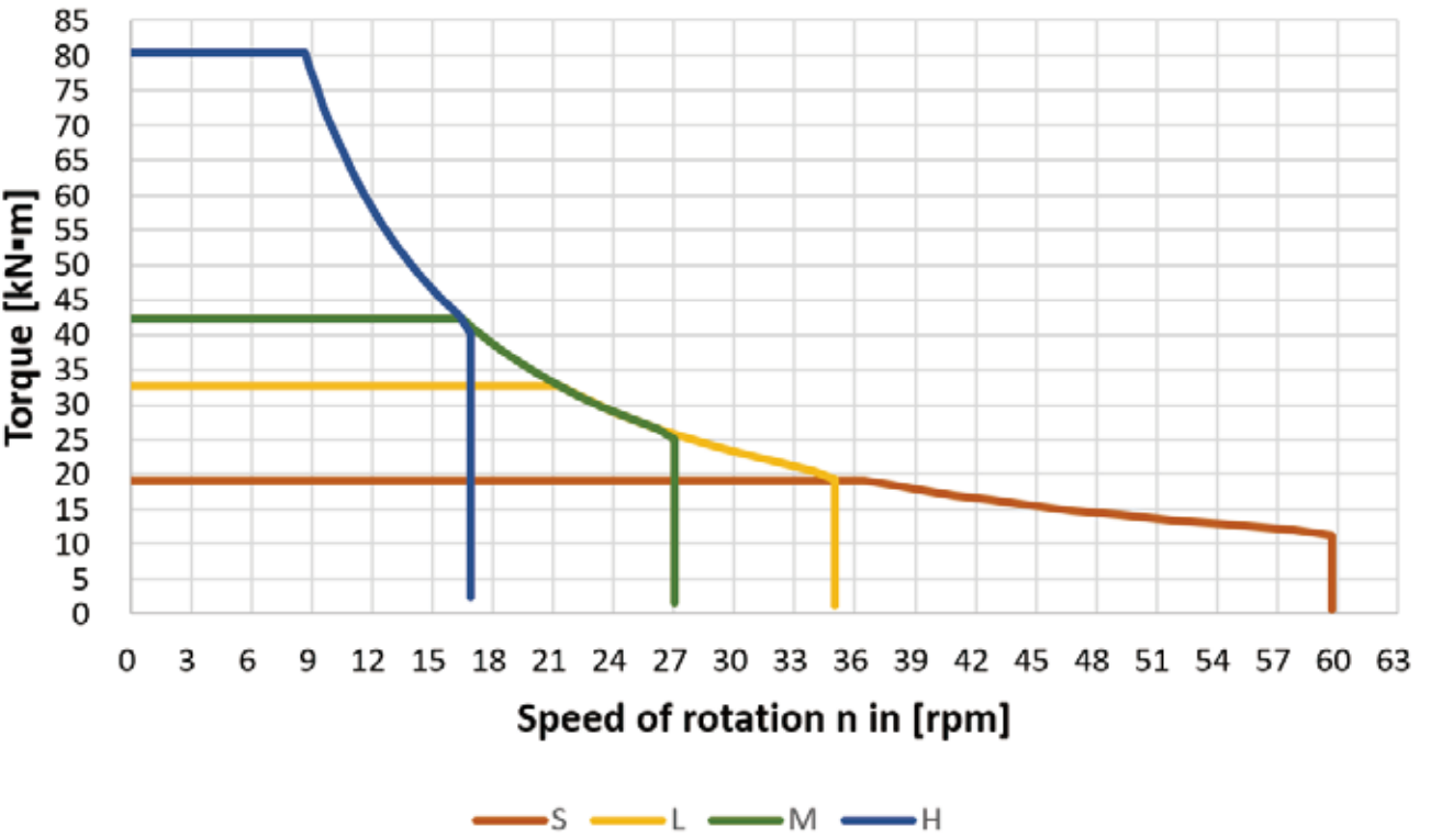
Rotary head
